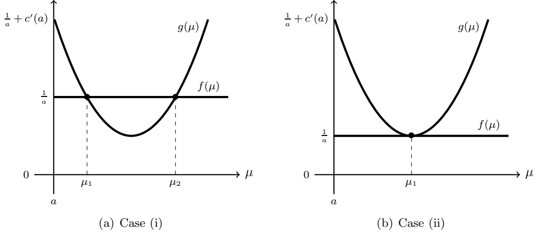
FIGURE EC.2. The limiting first order condition (16).
