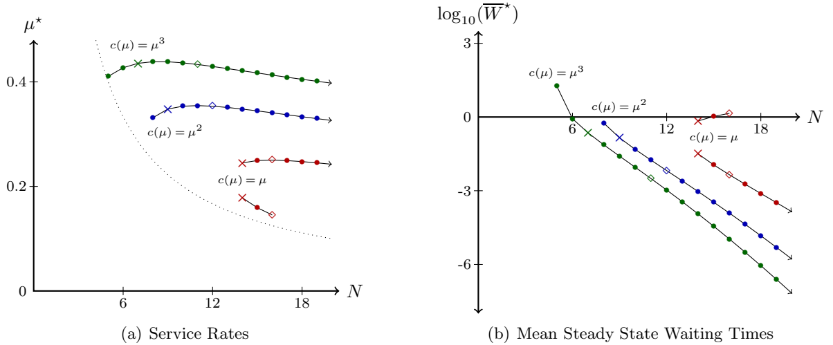
FIGURE 2. Equilibrium behavior as a function of the staffing level when the arrival rate is fixed at \lambda = 2 , for three different effort cost functions: linear, quadratic, and cubic. The dotted curve in (a) is \mu = \lambda/N = 2/N . The data points marked \times and \diamond correspond to N^{ao,2} and N^{opt,2} respectively.
