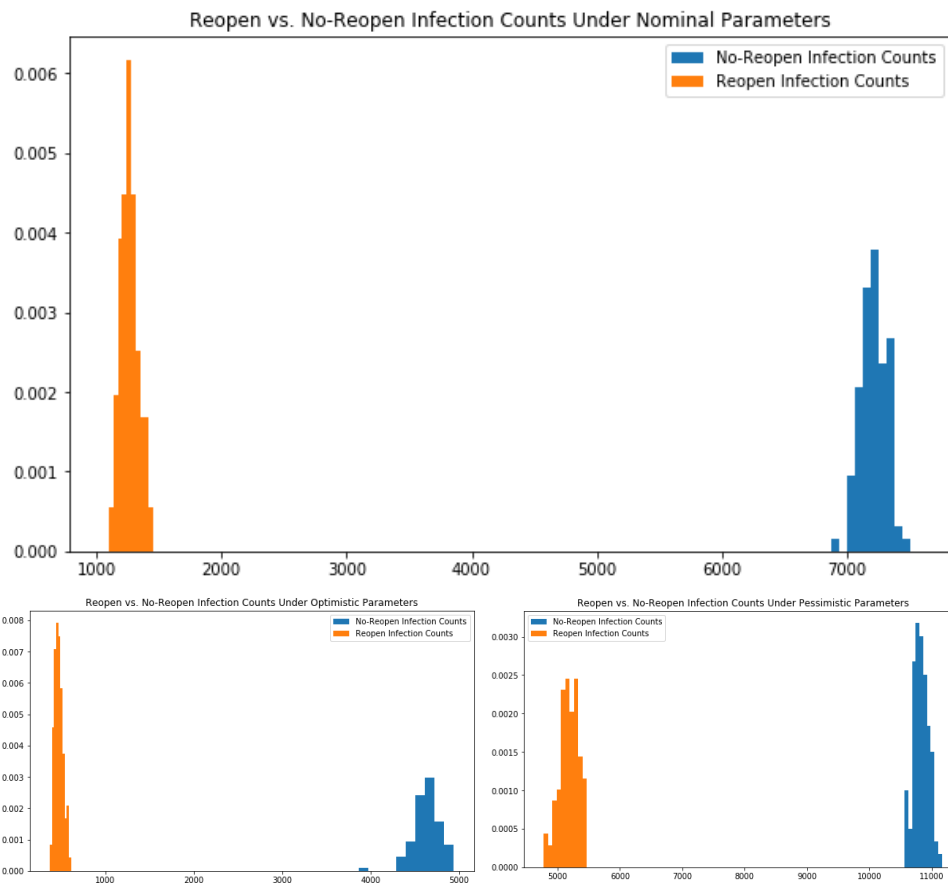
Figure 18: Histograms showing the number of infections in the fall semester under nominal, optimistic, and pessimistic variants of the Reopen vs. No-Reopen alternatives.
