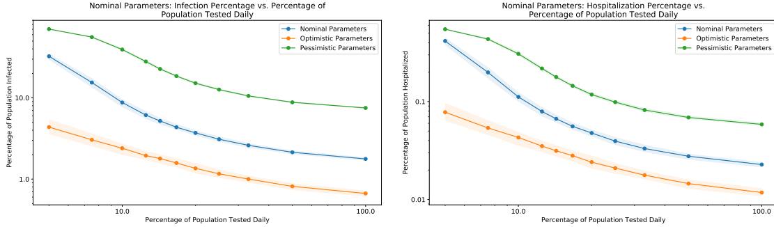
Figure 15: Plot depicts the distribution of infections and hospitalizations (i.e. 50th percentile, with the wider range corresponding to the 10-90th percentile range) vs. the percentage of the total population that is tested for the presence of infection each day. The value of this parameter is 20% of the population (across all scenarios), which approximately corresponds to testing the entire population once every 5 days. This was also shown above as Figure 5.
