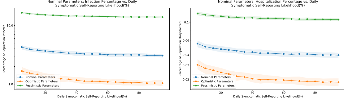
Figure 8: Plot depicts the distribution of infections and hospitalizations (i.e. 50th percentile, with the wider range corresponding to the 10-90th percentile range) vs. the daily likelihood that a symptomatic individual self-reports their infection status. The value of this parameter is 18%, for all the nominal/optimistic/pessimistic parameter scenarios.
