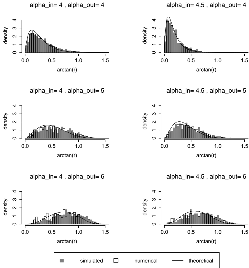
FIGURE 2. Comparison of the true density with the estimated densities of \arctan R over various values of (\alpha_{in}, \alpha_{out}) .
