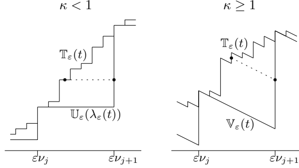
FIGURE 1. A demonstration of the matching of the parameterizations of the completed graphs of \mathbb{T}_\varepsilon with the completed graphs of \mathbb{U}_\varepsilon \circ \lambda_\varepsilon and \mathbb{V}_\varepsilon when \kappa \in (0, 1) and \kappa \in [1, 2) , respectively.
