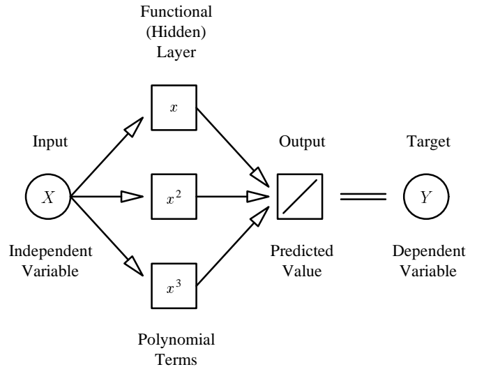
Figure 6: Functional Link Network = Polynomial Regression
