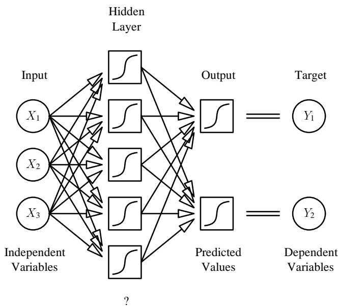
Figure 8: Multilayer Perceptron = Multivariate Multiple Nonlinear Regression
