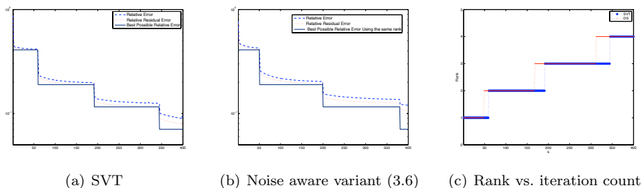
FIG. 5.2. Computational results for the city-to-city distance dataset. (a) Plot of the reconstruction errors from of the SVT algorithm. The blue dashed line is the relative error \|\mathbf{X}^k - \mathbf{M}\|_F / \|\mathbf{M}\|_F , the red dotted line is the relative residual error \|\mathcal{P}_\Omega(\mathbf{X}^k - \mathbf{M})\|_F / \|\mathcal{P}_\Omega(\mathbf{M})\|_F and the black line is the best possible relative error achieved by truncating the SVD of \mathbf{M} and keeping a number of terms equal to the rank of \mathbf{X}^k . (b) Same as (a) but with the iteration (3.6). (c) Rank of the successive iterates \mathbf{X}^k ; the SVT algorithm is in blue and the noise aware variant (3.6) is in red.
