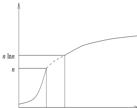
Complexity of convex minimization over an n -dimensional Euclidean ball
