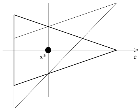
Partitioning of a pie and the induced partitioning of the symmetrized pie
