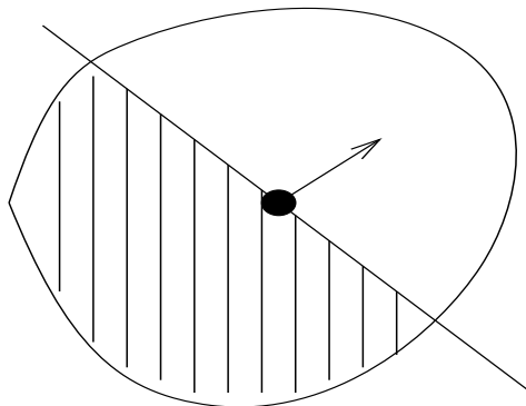
A step of a cutting plane method. Dashed region is the new localizer
