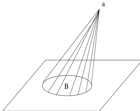
A conic set: B -base, a - vertex
